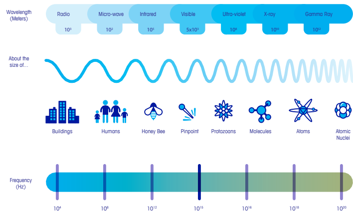
Figure 1: Electromagnetic Spectrum
