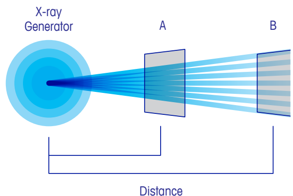
Figure 6 : Radiation intensity
