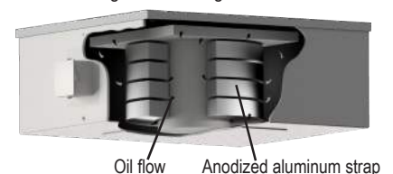
Dings Electromagnetic Coil
